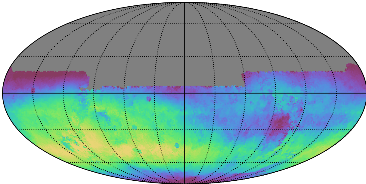
no_magell_roll_v3.4_10yrs All sky u band: Median skyBrightness
