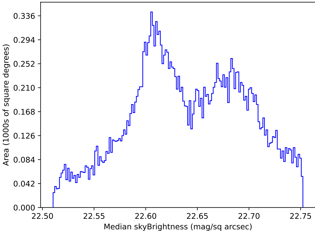
no_magell_roll_v3.4_10yrs All sky u band: Median skyBrightness
