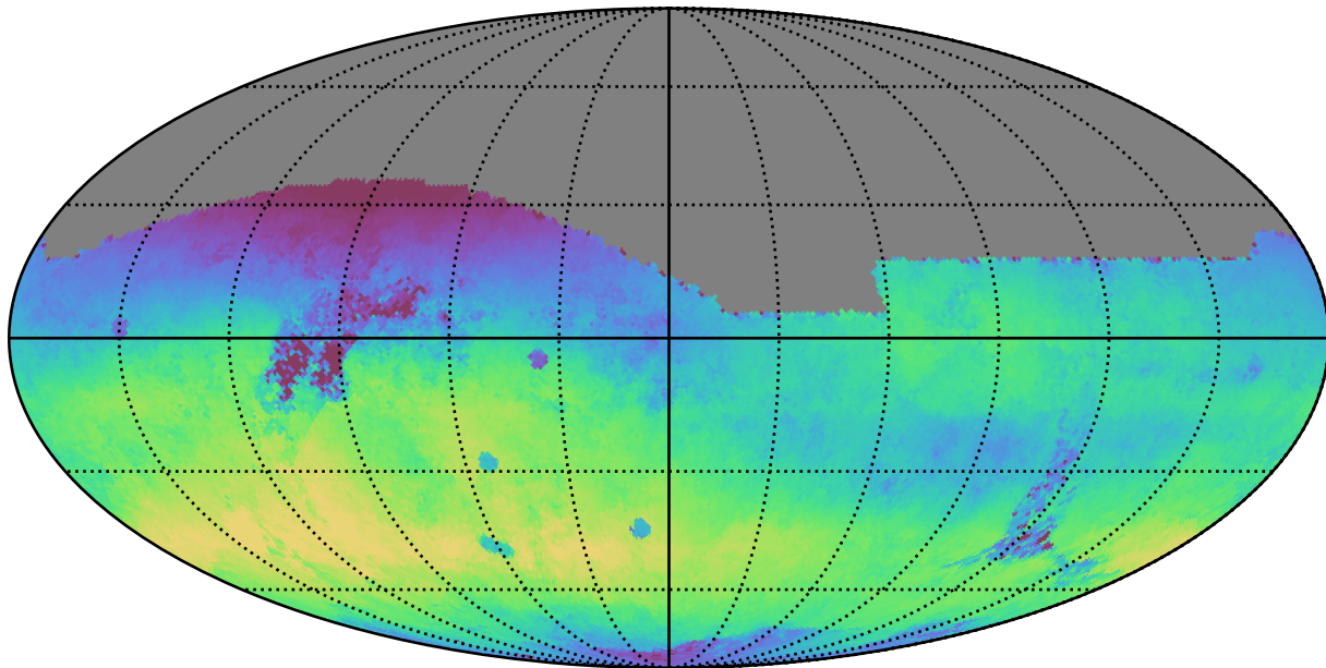
no_magell_roll_v3.4_10yrs All sky r band: Median skyBrightness
