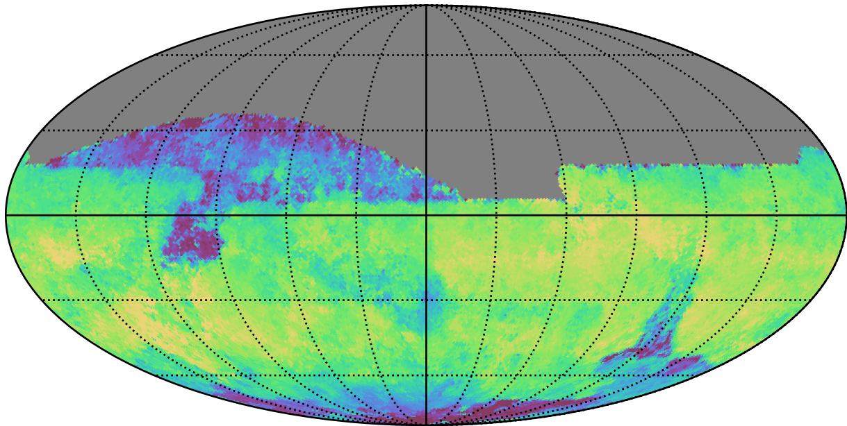
no_magell_roll_v3.4_10yrs All sky i band: Median skyBrightness
