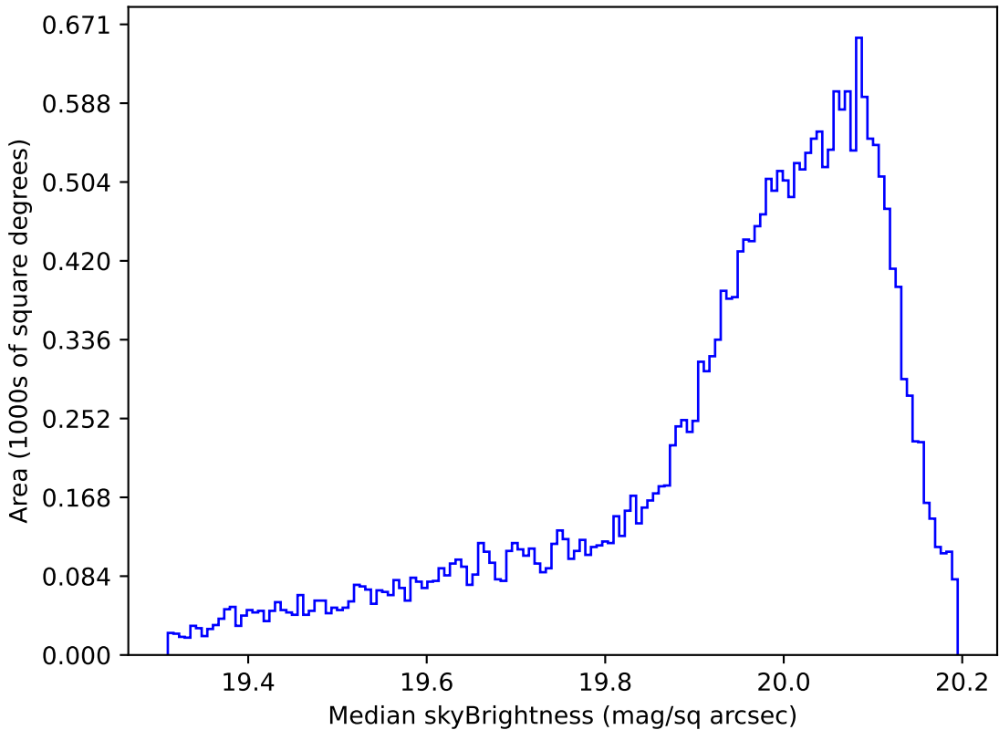
no_magell_roll_v3.4_10yrs All sky i band: Median skyBrightness
