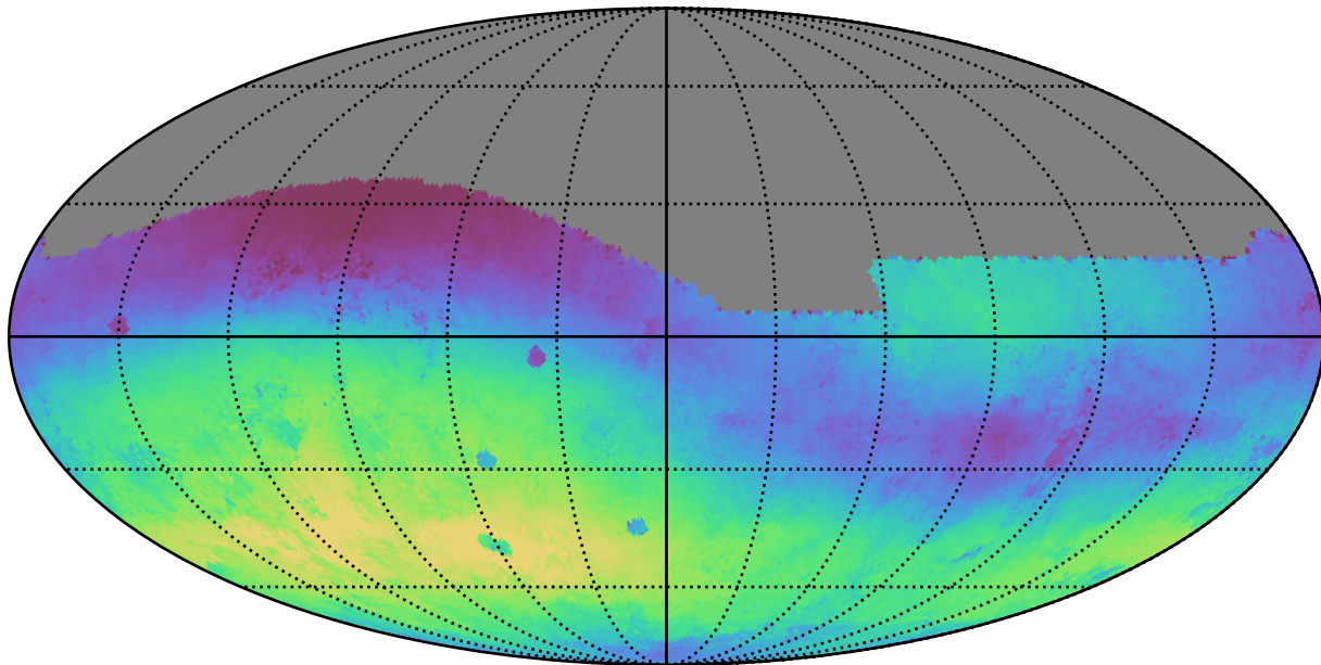
no_magell_roll_v3.4_10yrs All sky g band: Median skyBrightness
