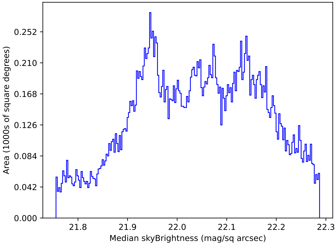
no_magell_roll_v3.4_10yrs All sky g band: Median skyBrightness
