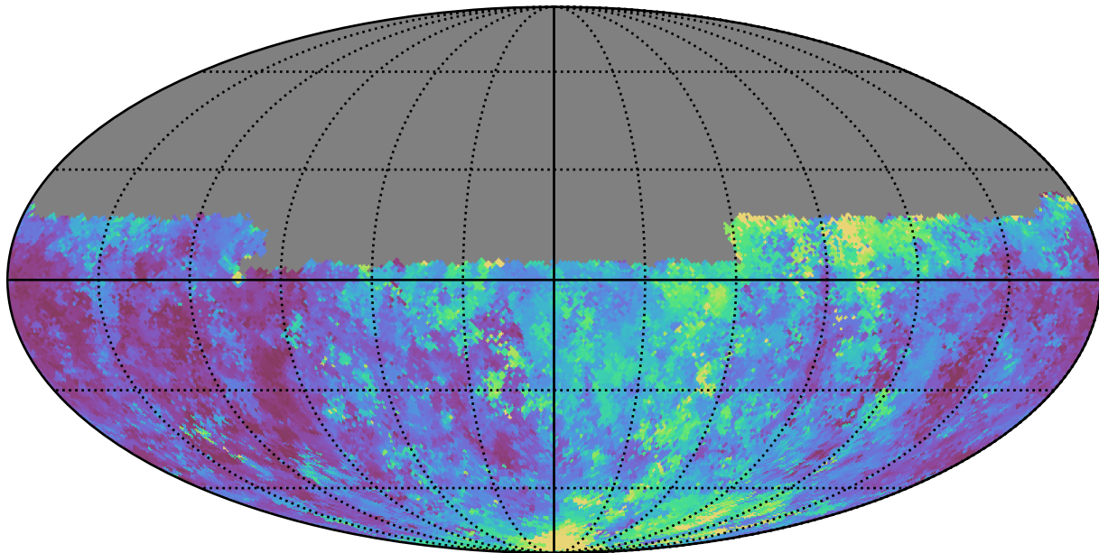
no_magell_roll_v3.4_10yrs Yr 1 u band: Median seeingGeom
