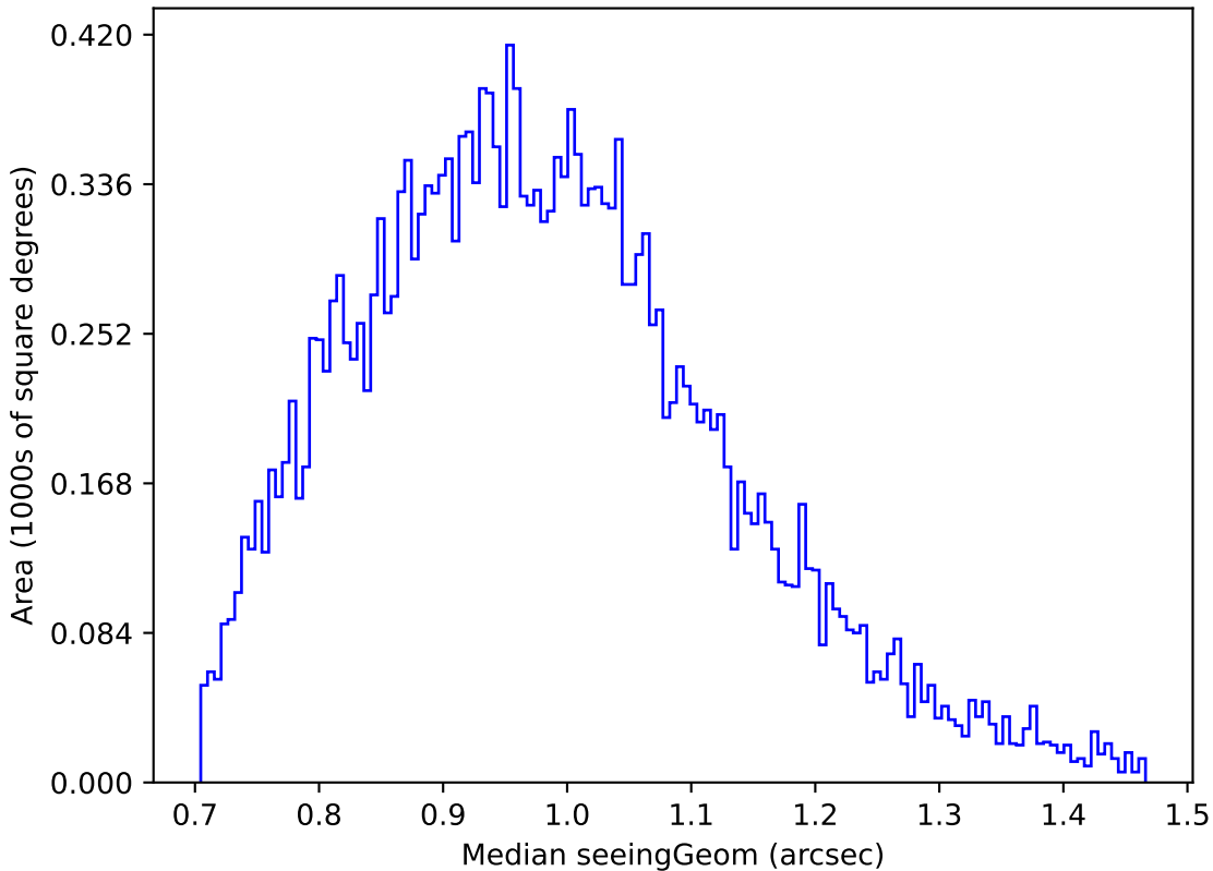
no_magell_roll_v3.4_10yrs Yr 1 u band: Median seeingGeom
