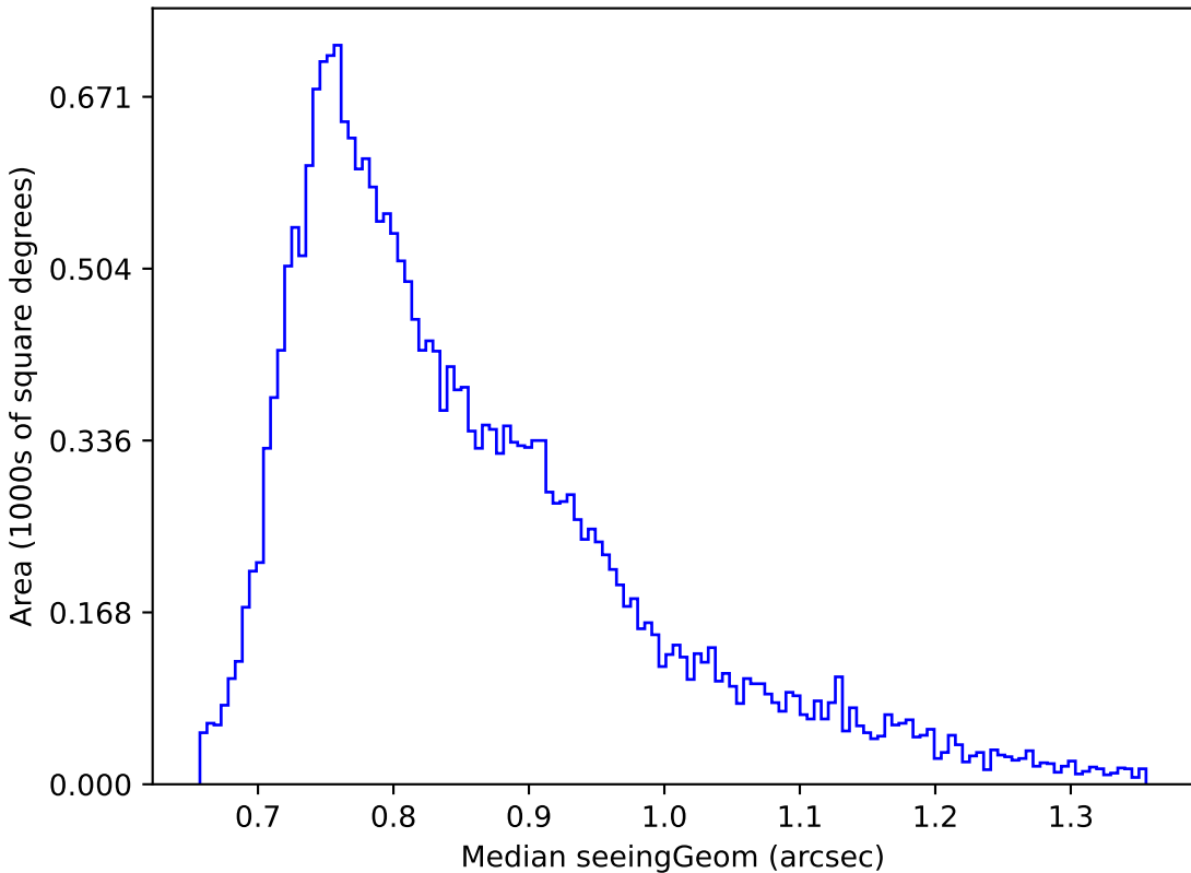
no_magell_roll_v3.4_10yrs Yr 1 r band: Median seeingGeom
