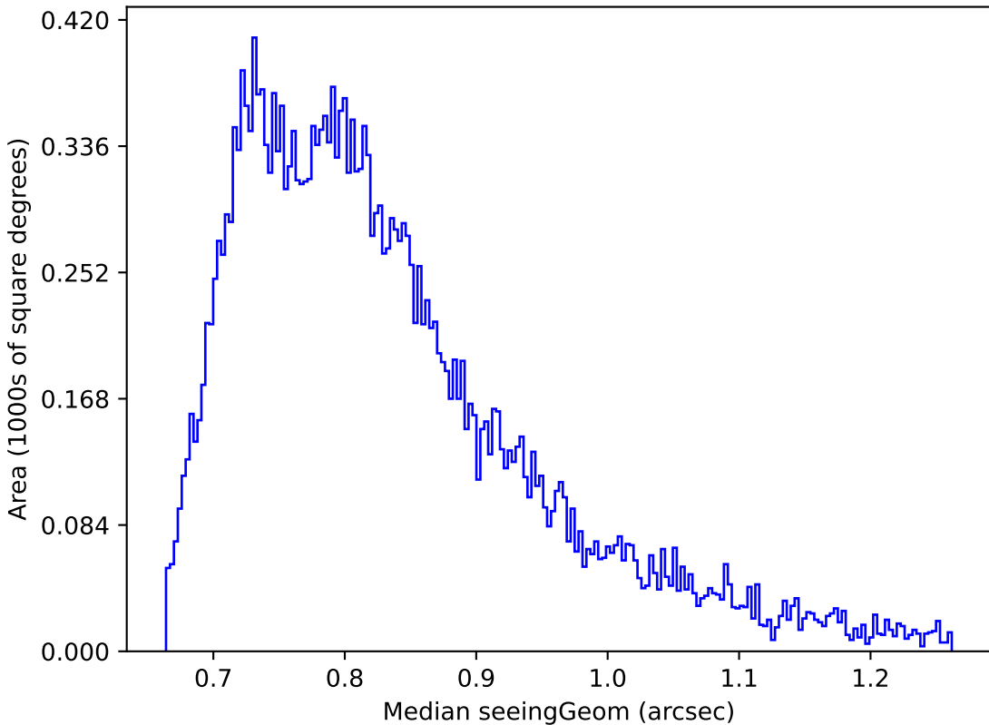
no_magell_roll_v3.4_10yrs Yr 1 i band: Median seeingGeom
