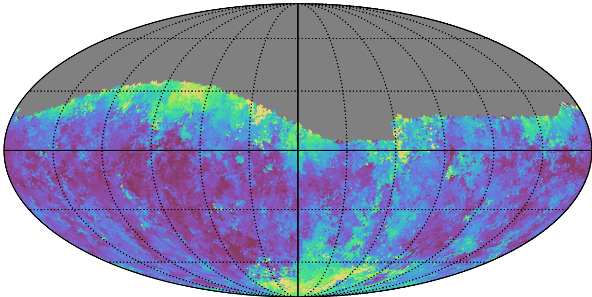
no_magell_roll_v3.4_10yrs Yr 1 g band: Median seeingGeom
