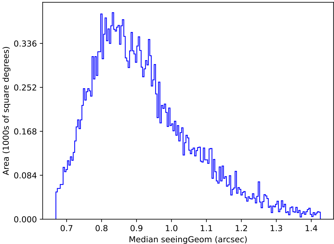
no_magell_roll_v3.4_10yrs Yr 1 g band: Median seeingGeom
