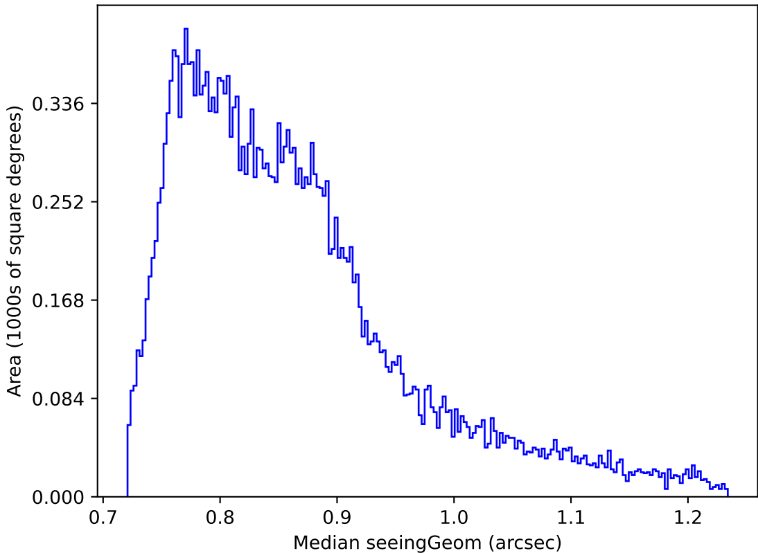
no_magell_roll_v3.4_10yrs Yr 1 all bands: Median seeingGeom
