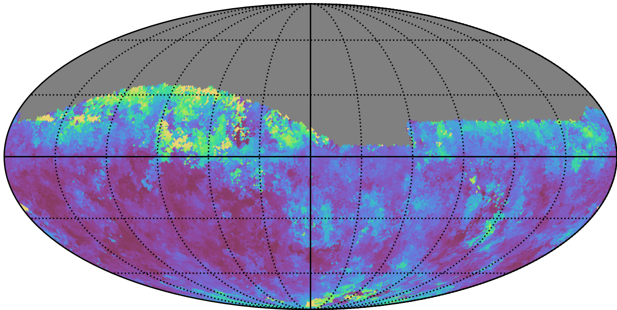
no_magell_roll_v3.4_10yrs Yr 1 z band: Median seeingEff
