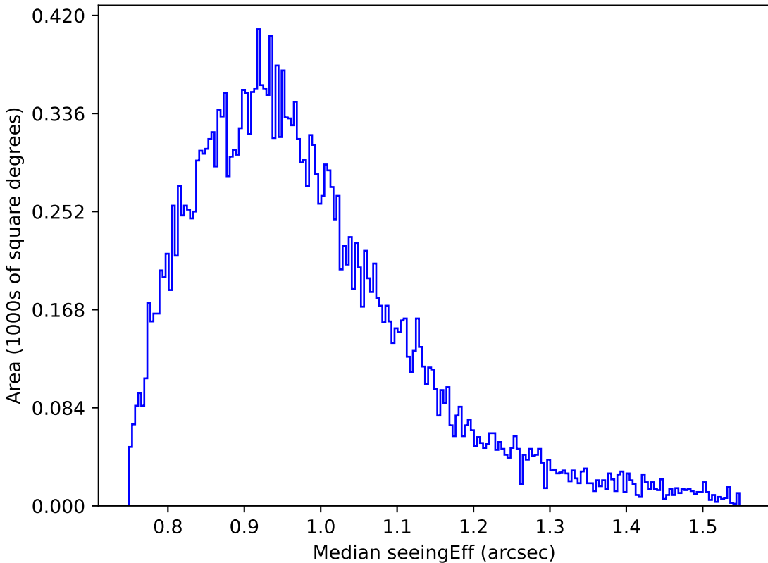
no_magell_roll_v3.4_10yrs Yr 1 z band: Median seeingEff
