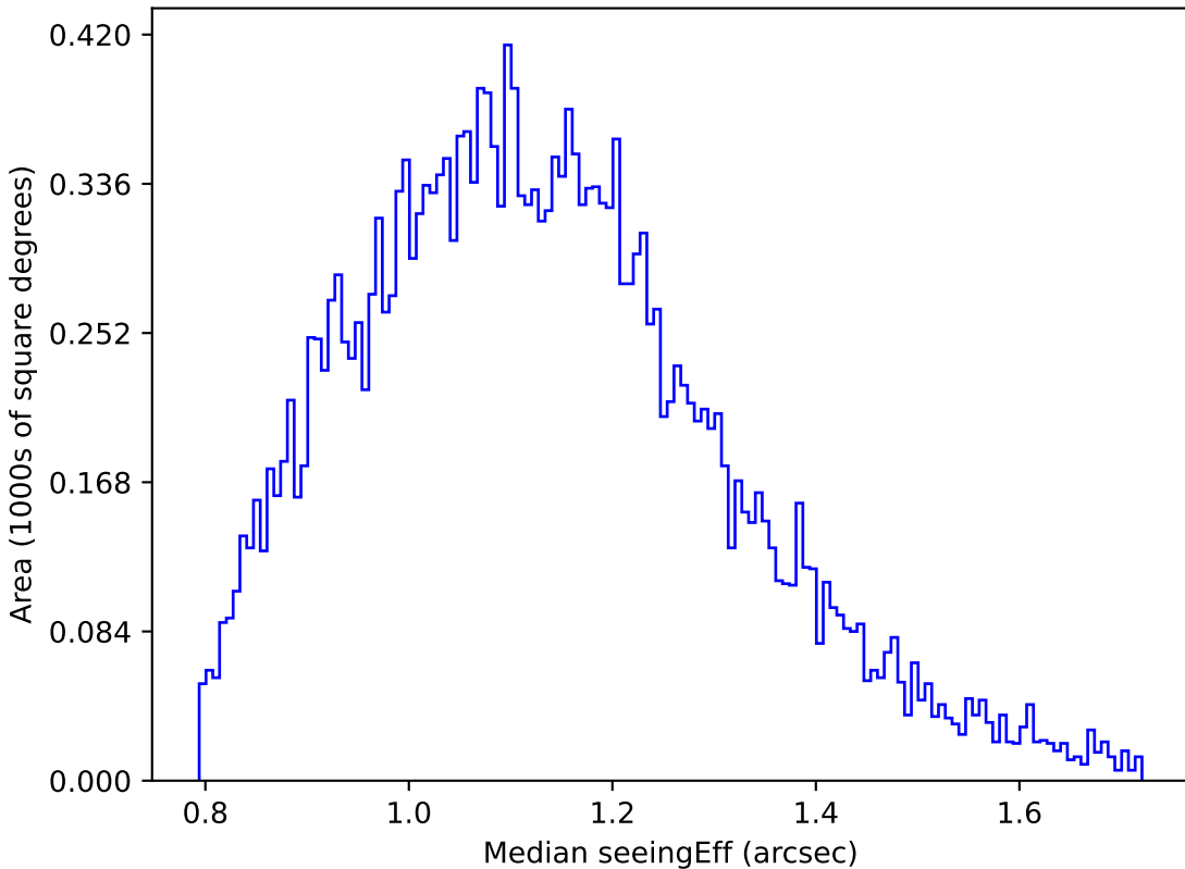
no_magell_roll_v3.4_10yrs Yr 1 u band: Median seeingEff
