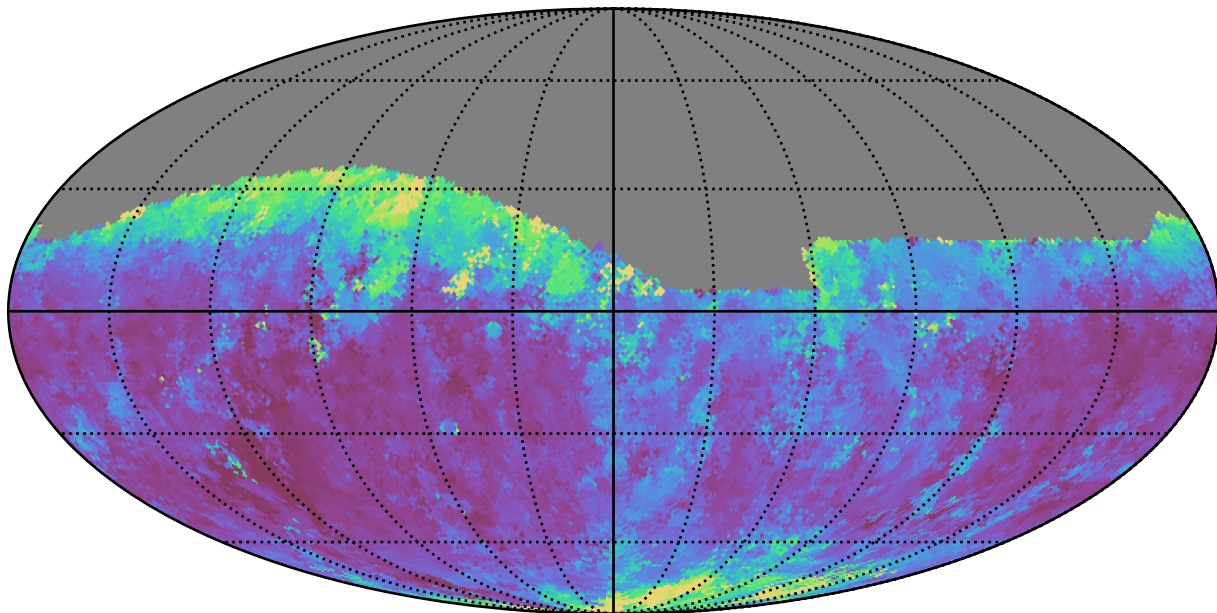
no_magell_roll_v3.4_10yrs Yr 1 r band: Median seeingEff
