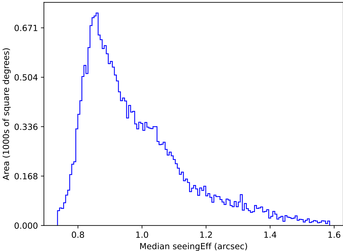
no_magell_roll_v3.4_10yrs Yr 1 r band: Median seeingEff
