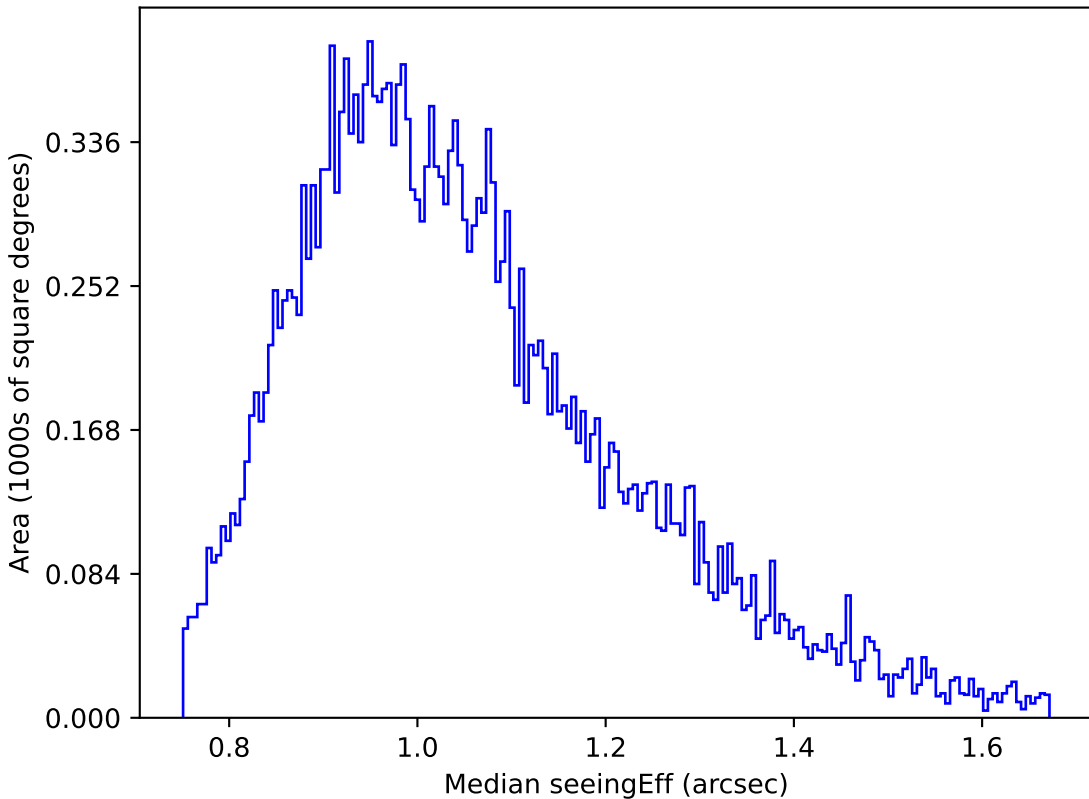
no_magell_roll_v3.4_10yrs Yr 1 g band: Median seeingEff
