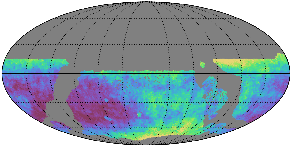
no_magell_roll_v3.4_10yrs WFD z band: Median seeingEff
