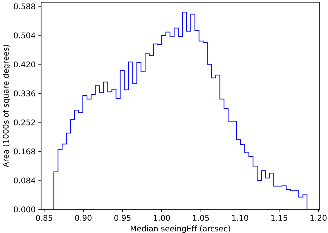
no_magell_roll_v3.4_10yrs WFD z band: Median seeingEff
