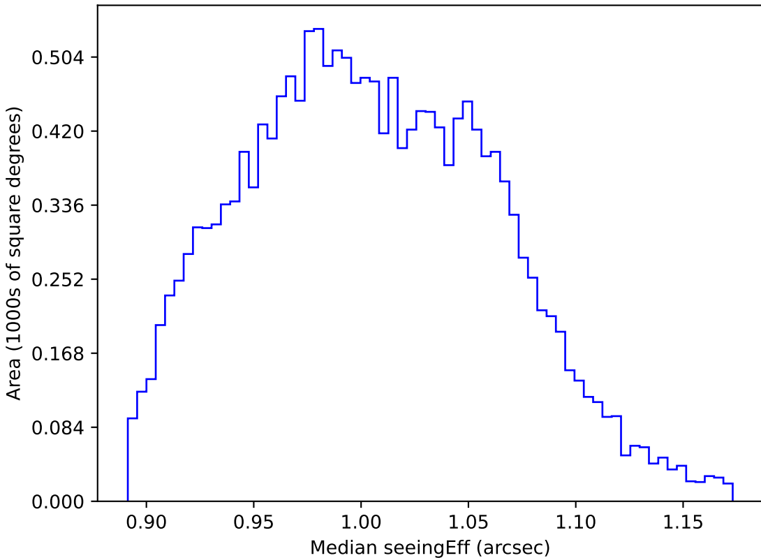
no_magell_roll_v3.4_10yrs WFD y band: Median seeingEff
