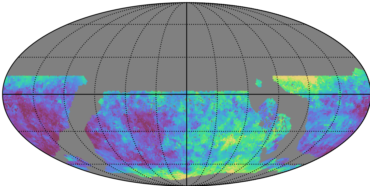
no_magell_roll_v3.4_10yrs WFD u band: Median seeingEff
