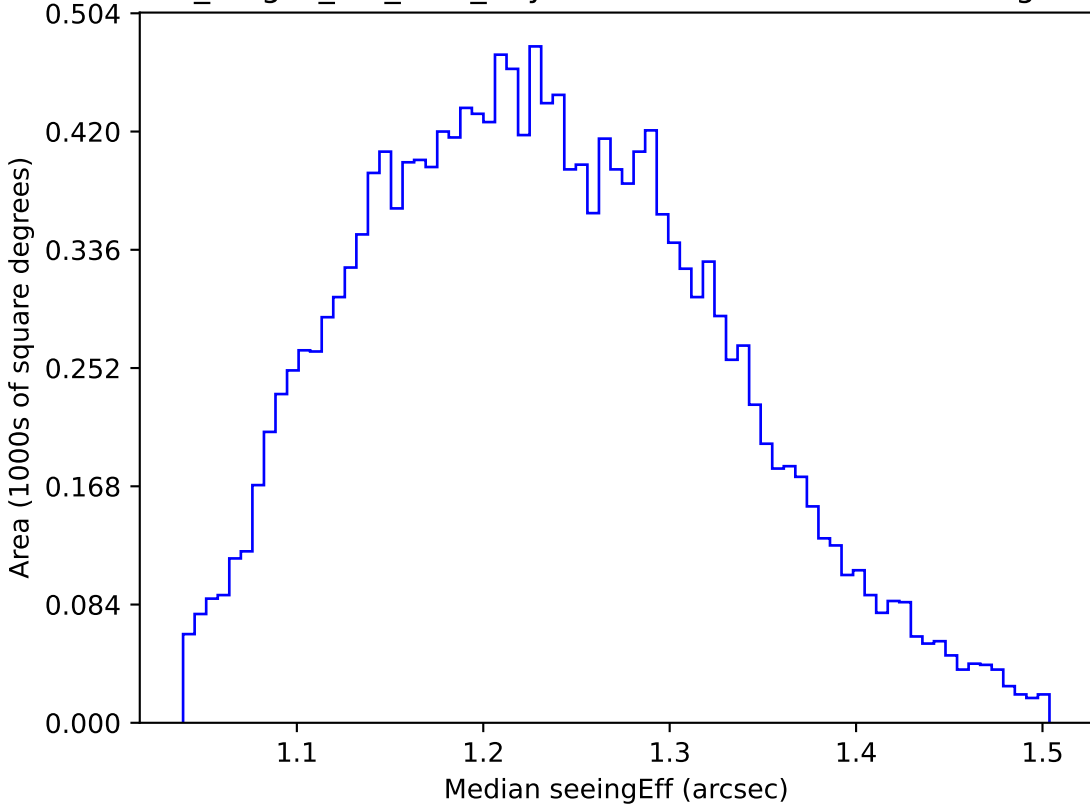
no_magell_roll_v3.4_10yrs WFD u band: Median seeingEff
