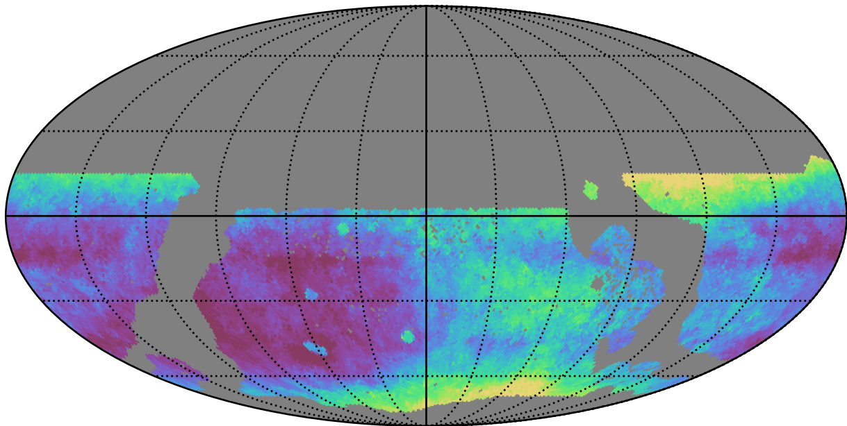
no_magell_roll_v3.4_10yrs WFD r band: Median seeingEff
