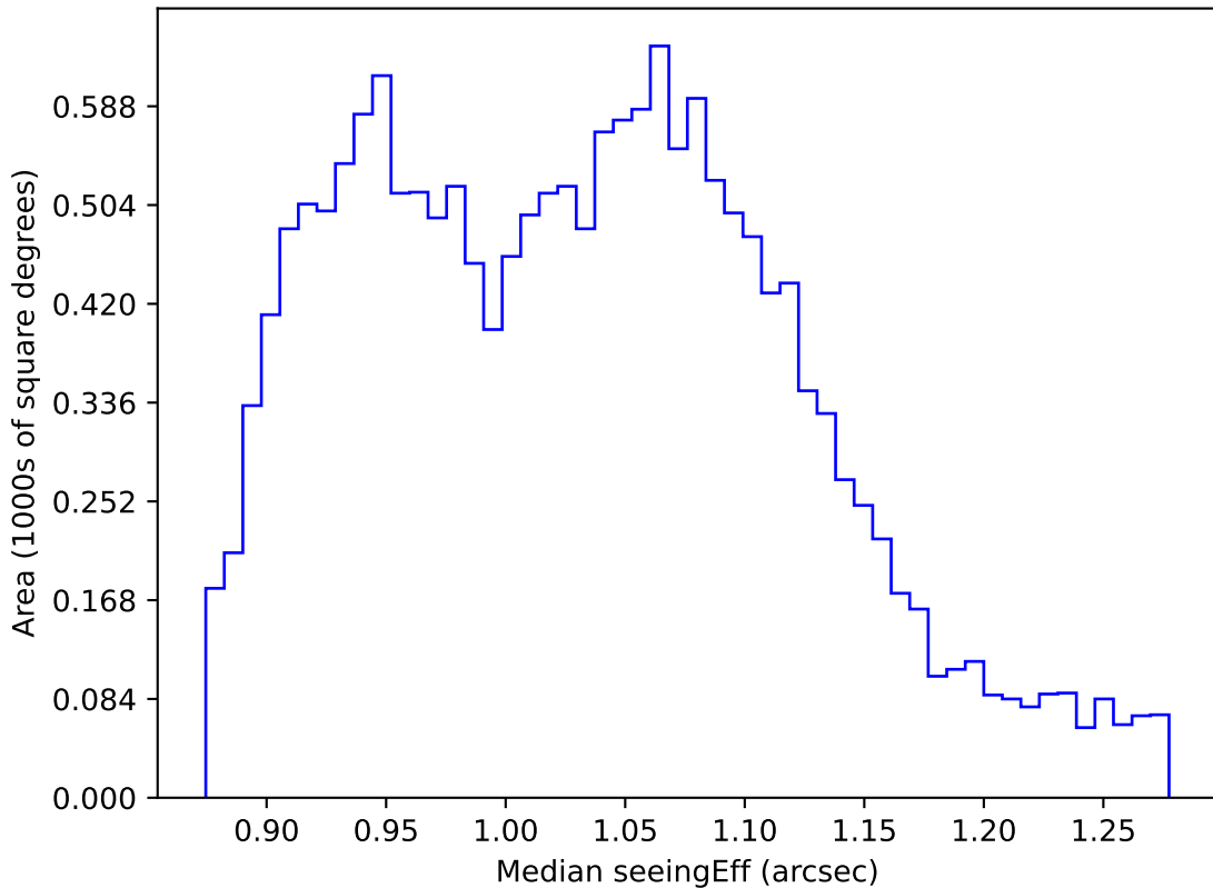
no_magell_roll_v3.4_10yrs WFD r band: Median seeingEff
