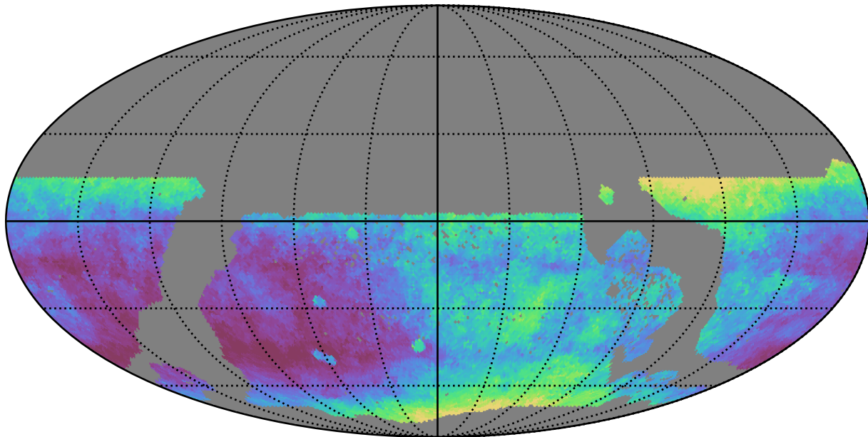
no_magell_roll_v3.4_10yrs WFD i band: Median seeingEff
