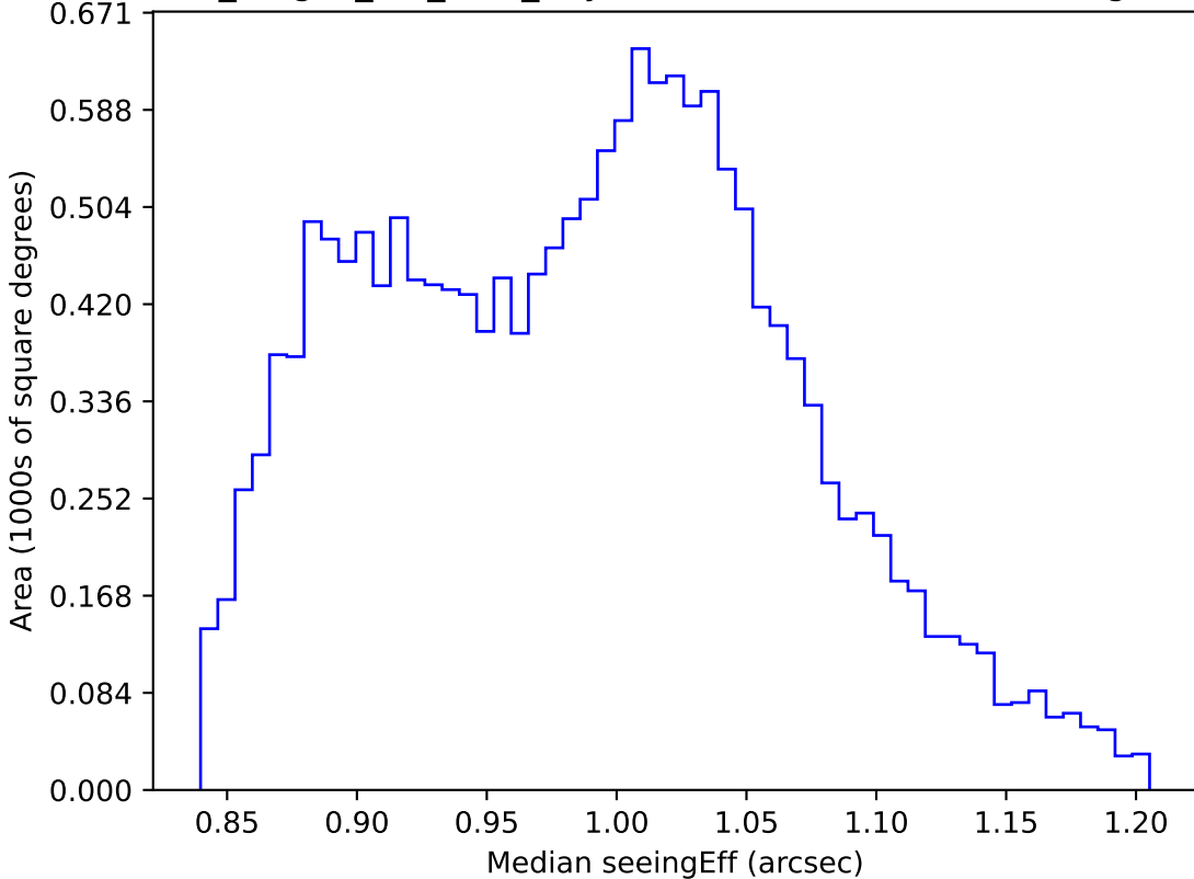
no_magell_roll_v3.4_10yrs WFD i band: Median seeingEff
