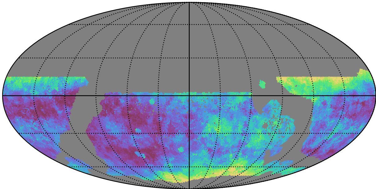
no_magell_roll_v3.4_10yrs WFD g band: Median seeingEff
