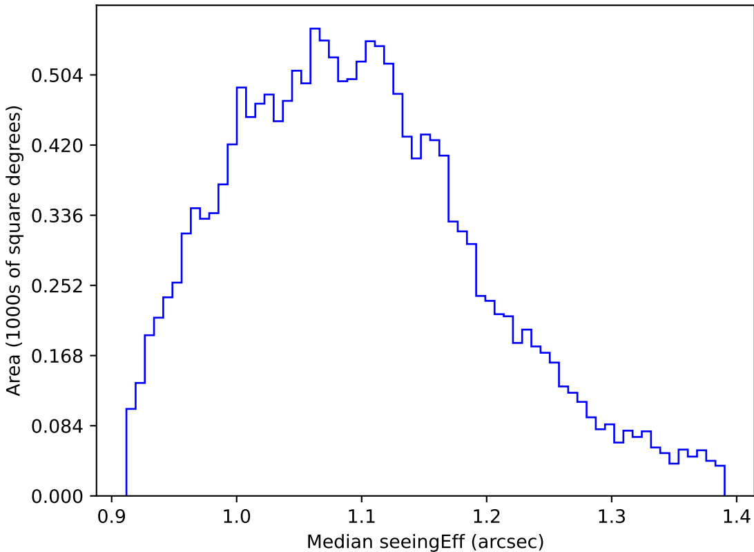
no_magell_roll_v3.4_10yrs WFD g band: Median seeingEff
