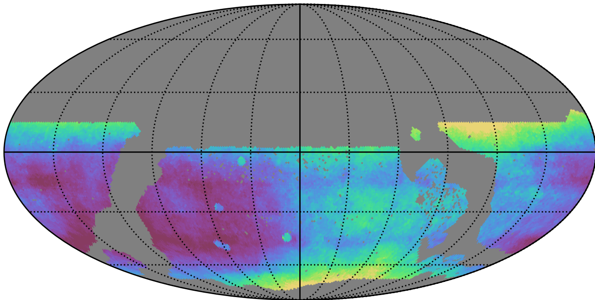
no_magell_roll_v3.4_10yrs WFD all bands: Median seeingEff
