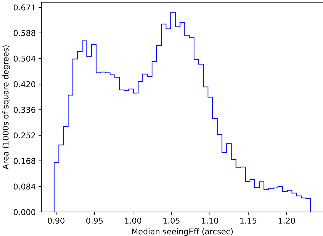
no_magell_roll_v3.4_10yrs WFD all bands: Median seeingEff
