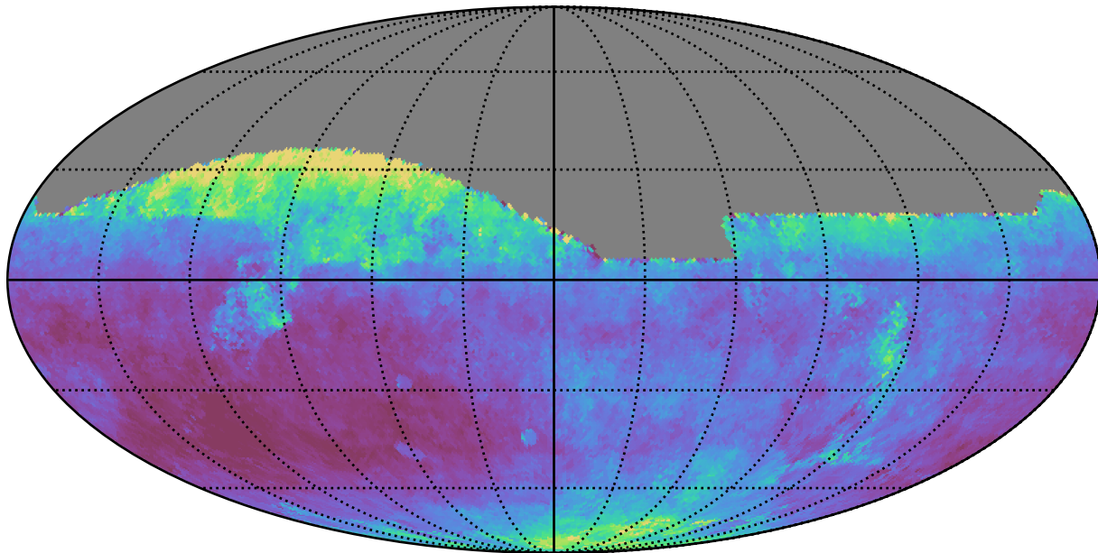
no_magell_roll_v3.4_10yrs All sky z band: Median seeingEff
