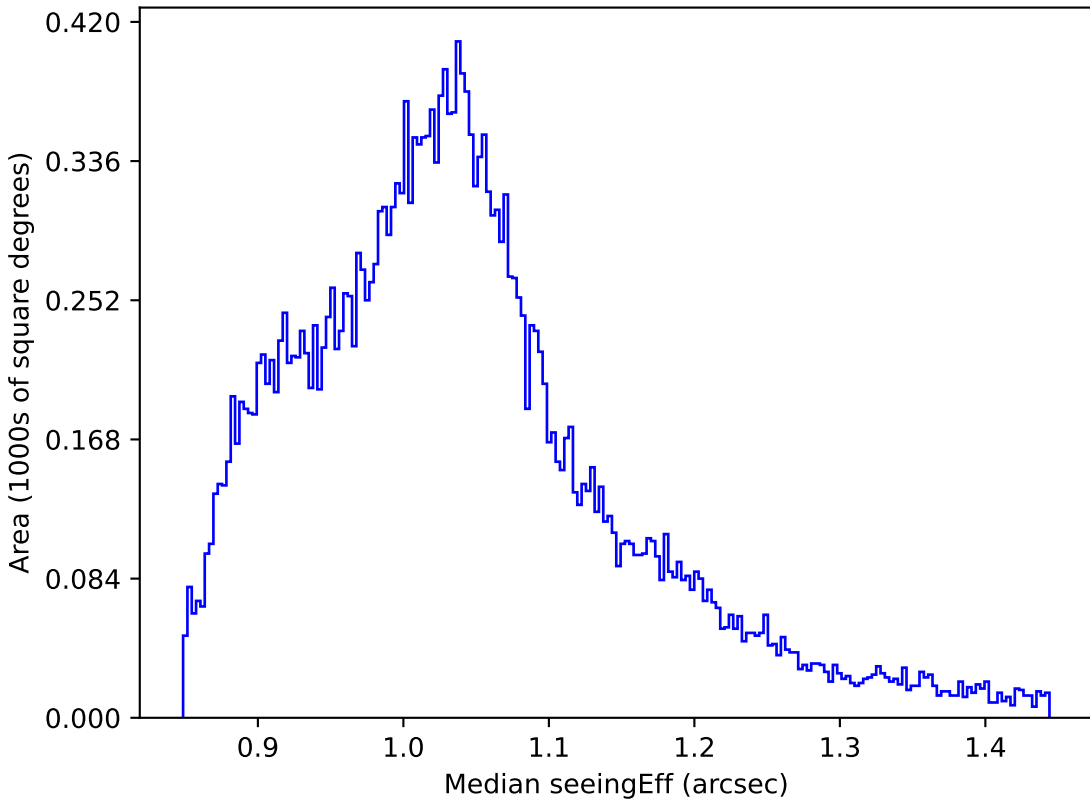
no_magell_roll_v3.4_10yrs All sky z band: Median seeingEff
