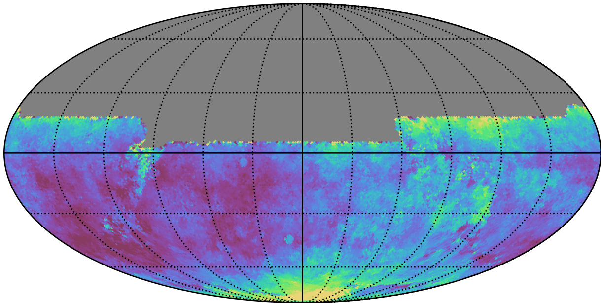
no_magell_roll_v3.4_10yrs All sky y band: Median seeingEff
