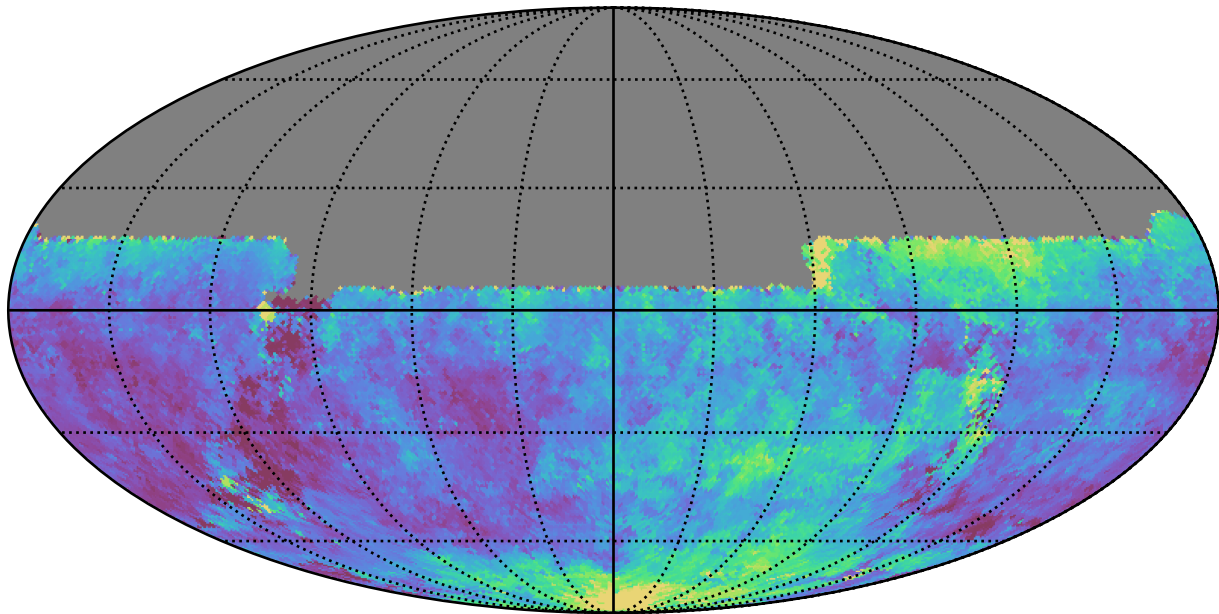
no_magell_roll_v3.4_10yrs All sky u band: Median seeingEff
