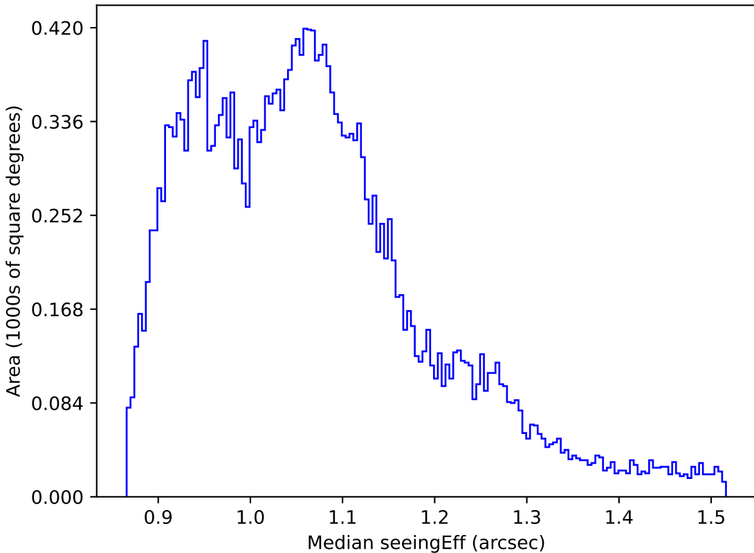
no_magell_roll_v3.4_10yrs All sky r band: Median seeingEff
