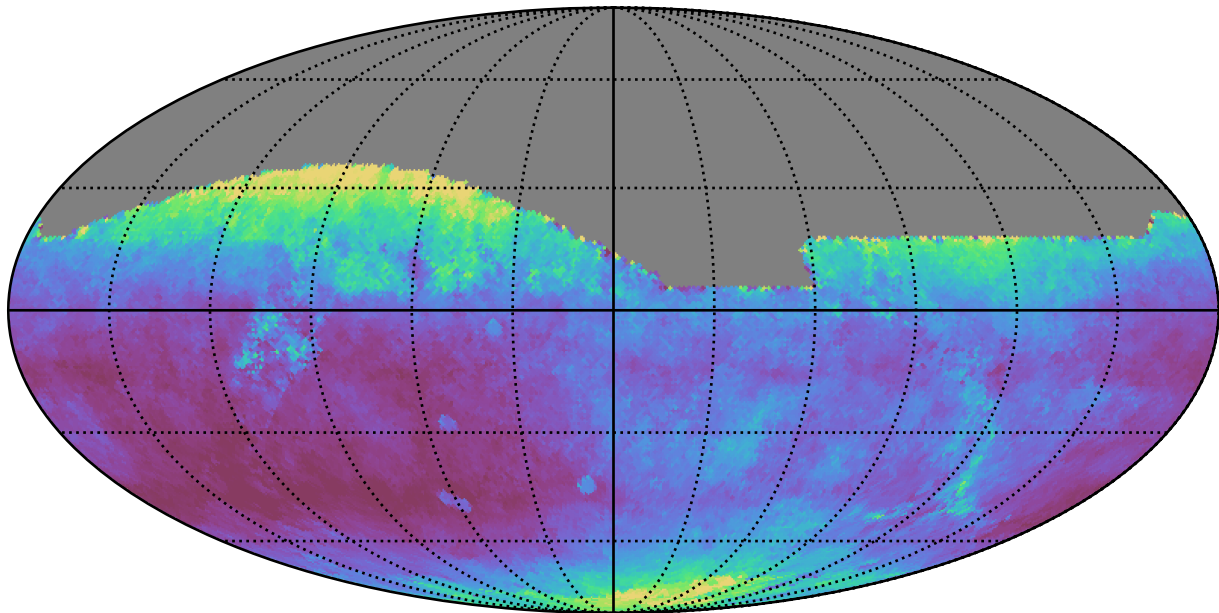
no_magell_roll_v3.4_10yrs All sky i band: Median seeingEff
