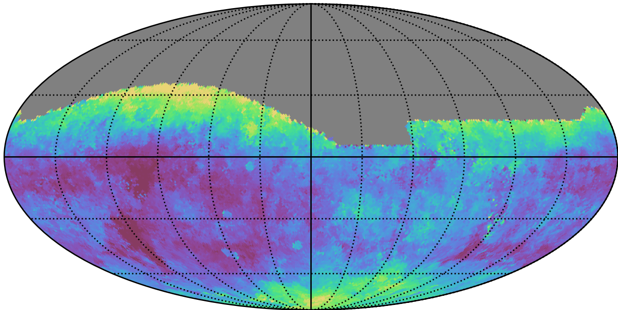
no_magell_roll_v3.4_10yrs All sky g band: Median seeingEff
