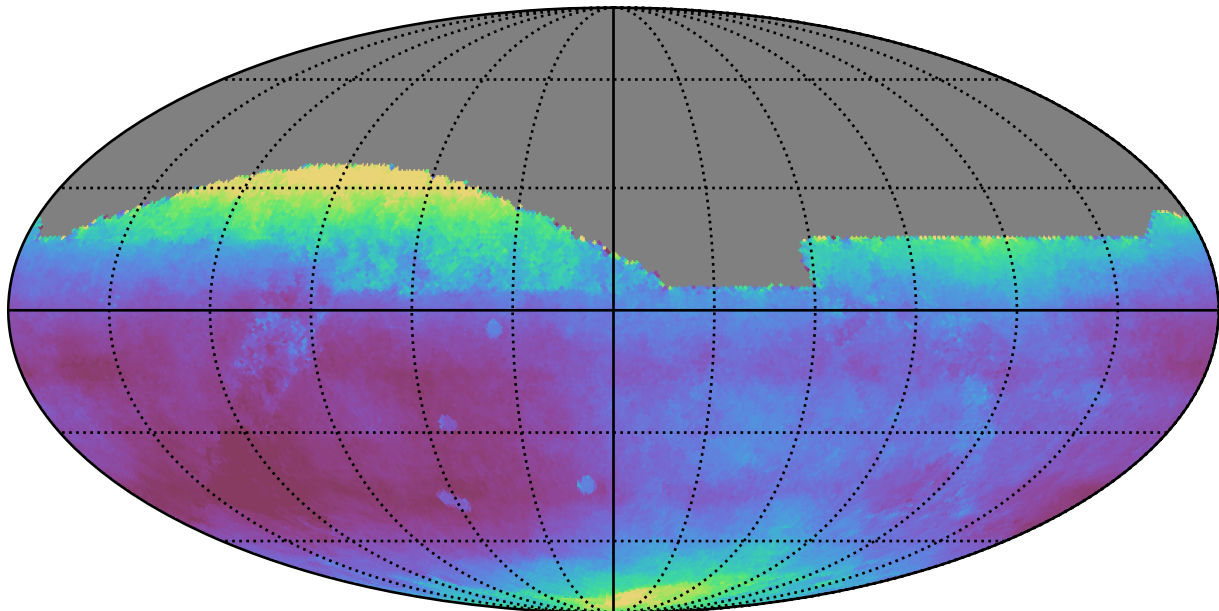
no_magell_roll_v3.4_10yrs All sky all bands: Median seeingEff
