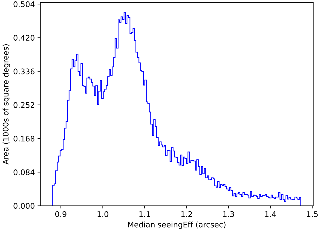
no_magell_roll_v3.4_10yrs All sky all bands: Median seeingEff
