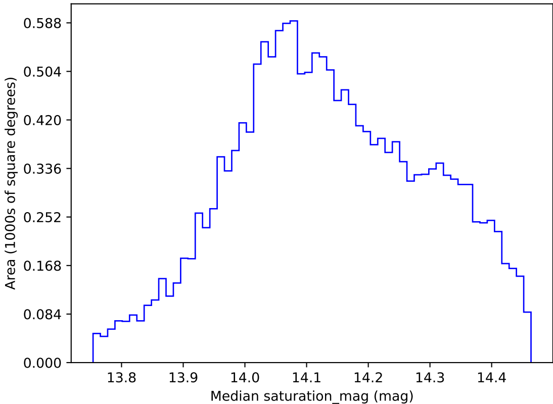
no_magell_roll_v3.4_10yrs WFD z band: Median saturation_mag
