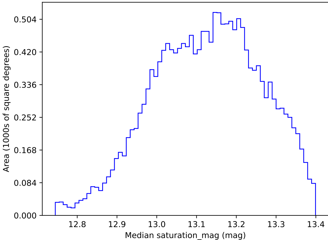
no_magell_roll_v3.4_10yrs WFD y band: Median saturation_mag
