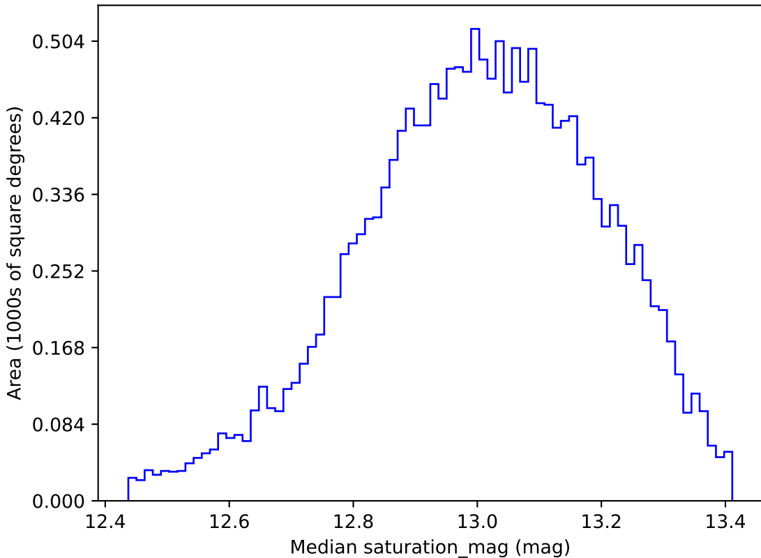
no_magell_roll_v3.4_10yrs WFD u band: Median saturation_mag
