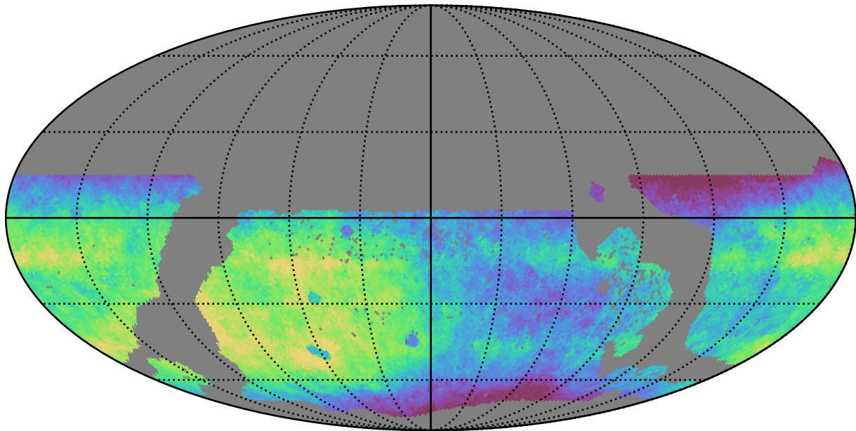
no_magell_roll_v3.4_10yrs WFD r band: Median saturation_mag
