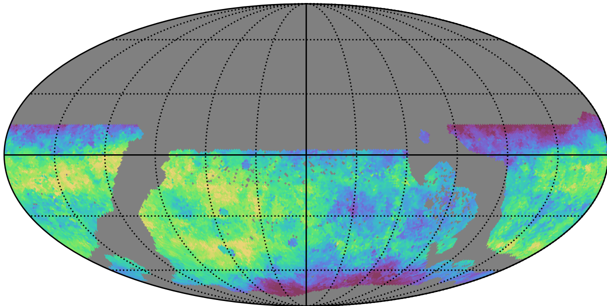
no_magell_roll_v3.4_10yrs WFD g band: Median saturation_mag
