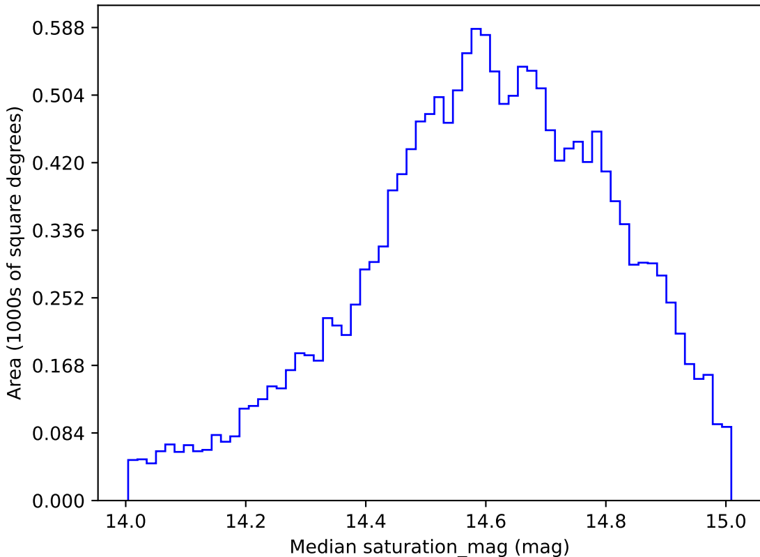
no_magell_roll_v3.4_10yrs WFD g band: Median saturation_mag
