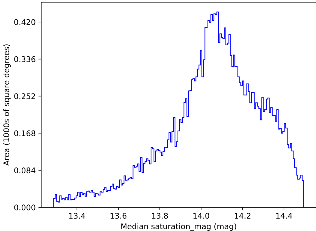
no_magell_roll_v3.4_10yrs All sky z band: Median saturation_mag
