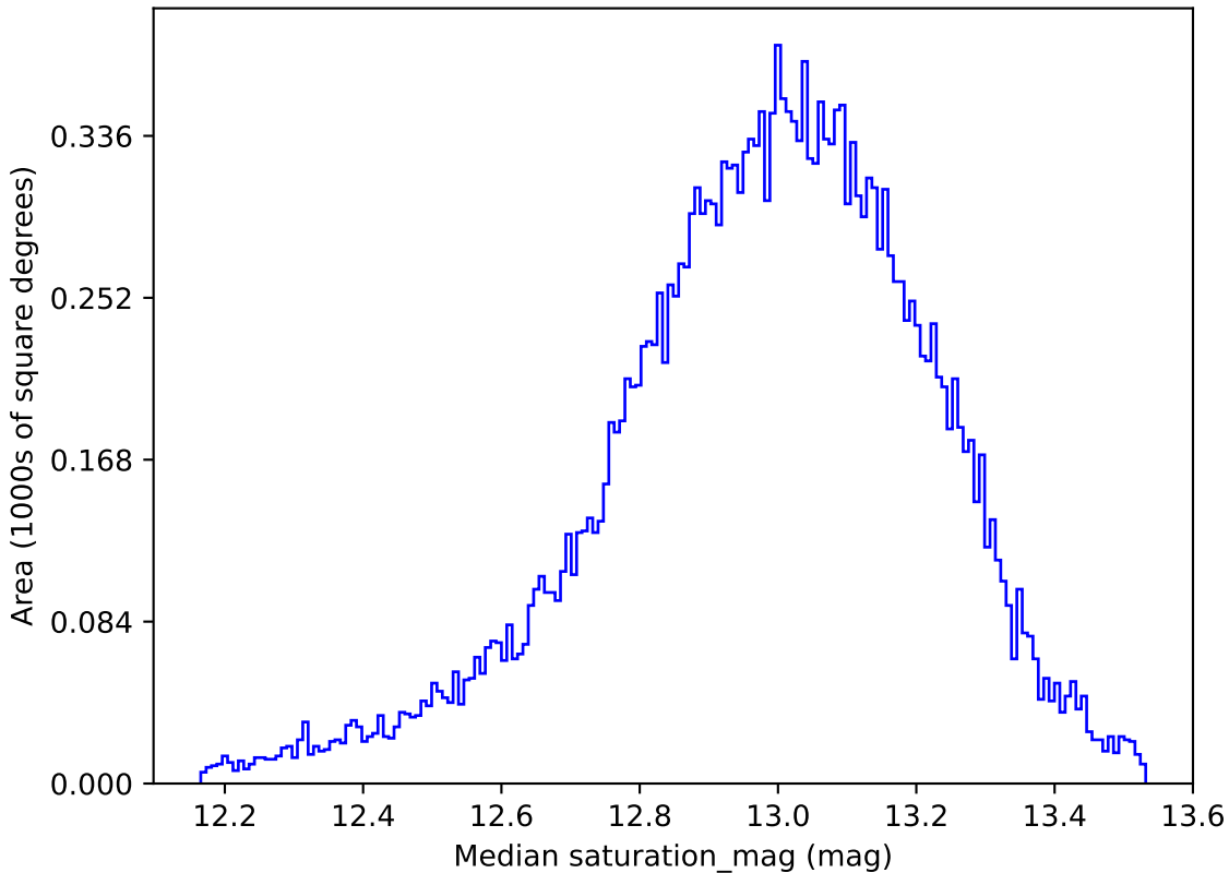
no_magell_roll_v3.4_10yrs All sky u band: Median saturation_mag
